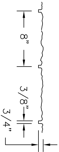
SECTION VIEW
