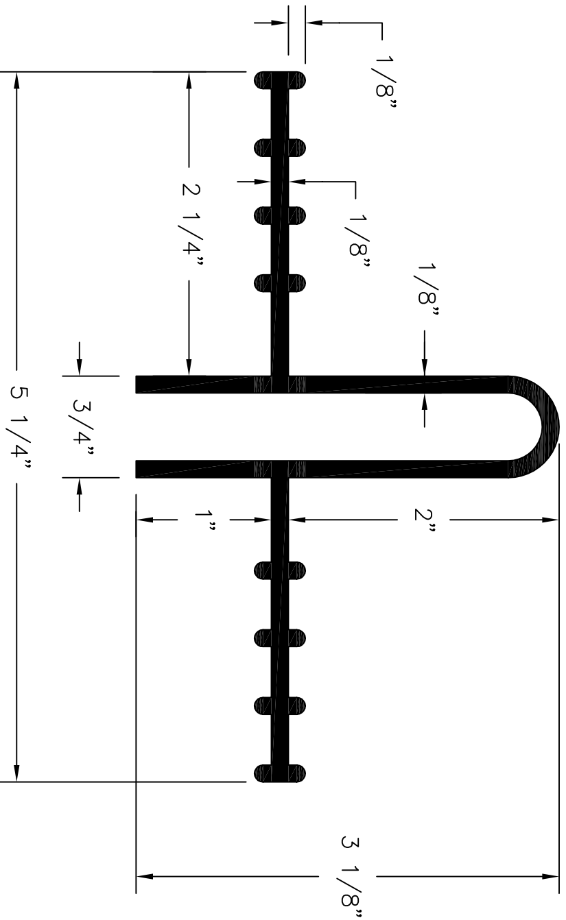
U550 PROFILE SCALE: NTS
